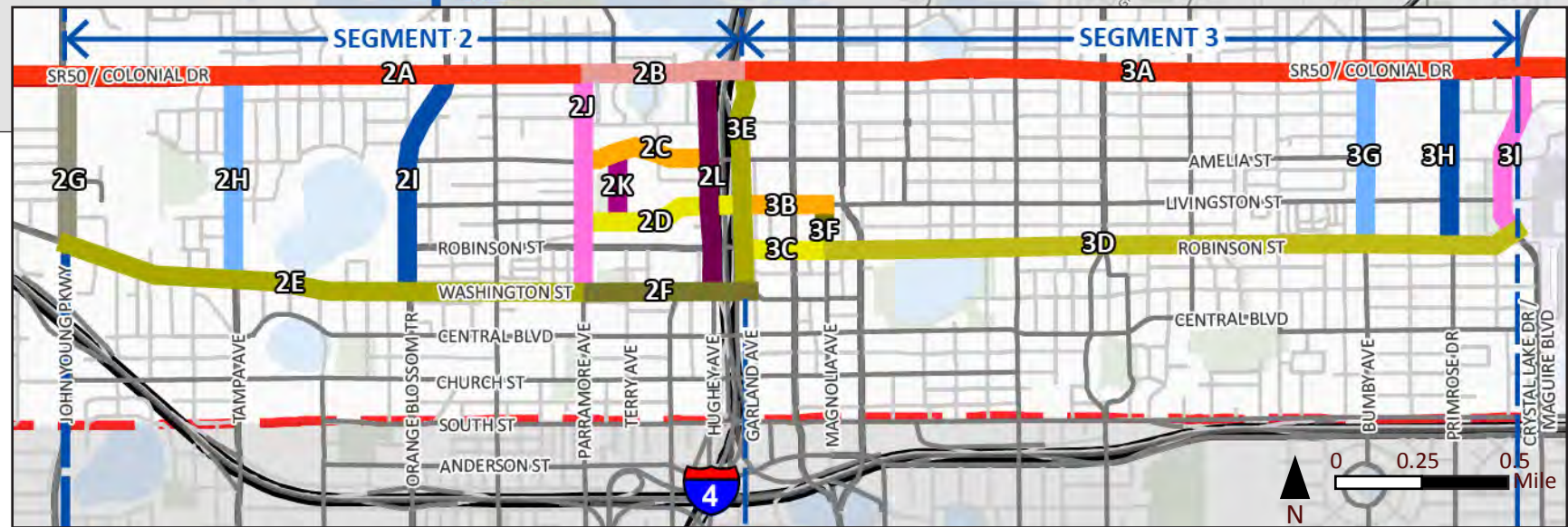
Segments 2 & 3 Alignments Alternatives
